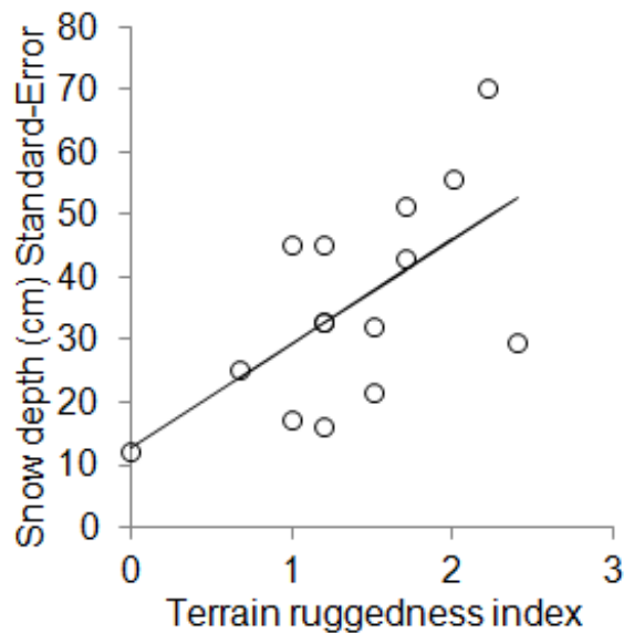
Figure 3.4 Variability in spring snow depth (cm) measured at 50 locations within each sampled quadrat ( 1 \text{ km}^2 ) on Herschel Island as a function of respective Terrain Ruggedness Index (TRI) values (Nellemann and Thomsen 1994) calculated for each quadrat. The linear regression is positive and statistically significant ( y = 12.59 + 16.68[\text{TRI}] , F_{1,13} = 8.17 , P = 0.01 , R^2 = 0.34 , n = 15 ).
