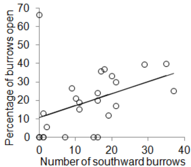
Figure 3.3 Percentage of burrows found to be open (unfrozen) in May of 2009 in relation to the number of burrows that are facing southward on each studied dens on Herschel Island. The linear regression is positive and statistically significant ( y = 10.53 + 0.66[\text{Number of southward burrows}] , F_{1,23} = 4.63 , P = 0.04 , R^2 = 0.13 , n = 25 ).
