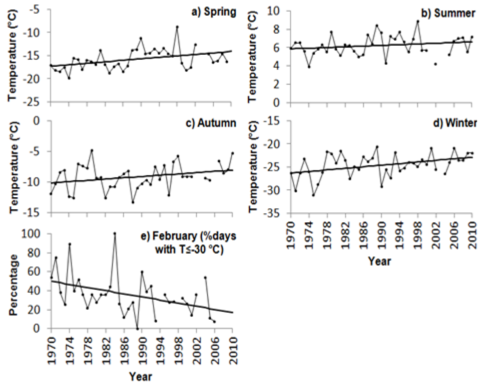
Figure 2.2 Meteorological data from Komakuk Beach Environment Canada weather station in the Yukon Coastal Plain, showing mean monthly air temperatures (1970–2010) for a) spring (temperature = 0.08[\text{year}] - 174.67 , F_{1,36} = 7.35 , P = 0.01 , R^2 = 0.17 , n = 38 ), b) summer (temperature = 0.02[\text{year}] - 31.62 , F_{1,36} = 1.53 , P = 0.22 , R^2 = 0.04 , n = 38 ), c) autumn (temperature = 0.05[\text{year}] - 113.81 , F_{1,36} = 3.49 , P = 0.07 , R^2 = 0.09 , n = 38 ), d) winter (temperature = 0.09[\text{year}] - 195.86 , F_{1,38} = 7.53 , P = 0.01 , R^2 = 0.17 , n = 40 ), and e) percentages of days in February when average daily air temperature was -30\text{ }^{\circ}\text{C} or less (1970–2006), indicating a statistically significant decline (percentage = 1668.00 - 0.82[\text{year}] , F_{1,32} = 6.30 , P = 0.02 , R^2 = 0.17 , n = 34 ).
